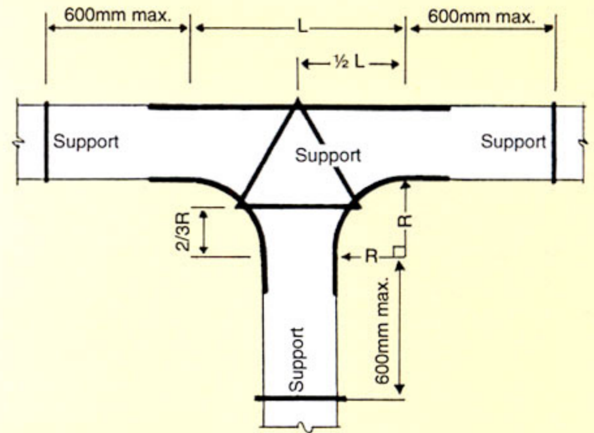
PLAN VIEW
