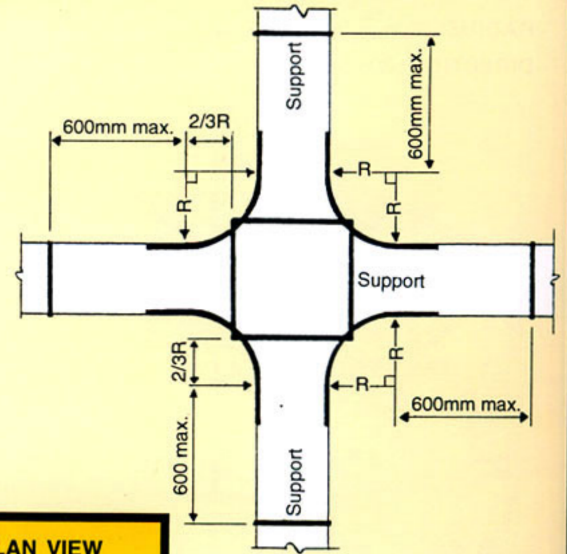
PLAN VIEW
