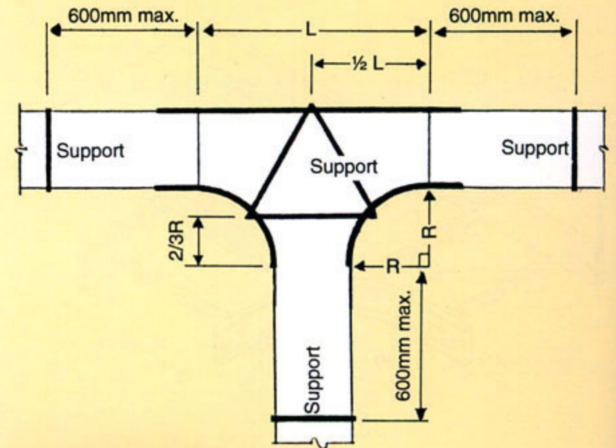
PLAN VIEW
