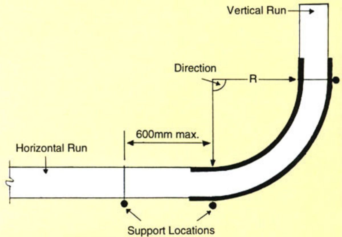
ELEVATIONAL VIEW
