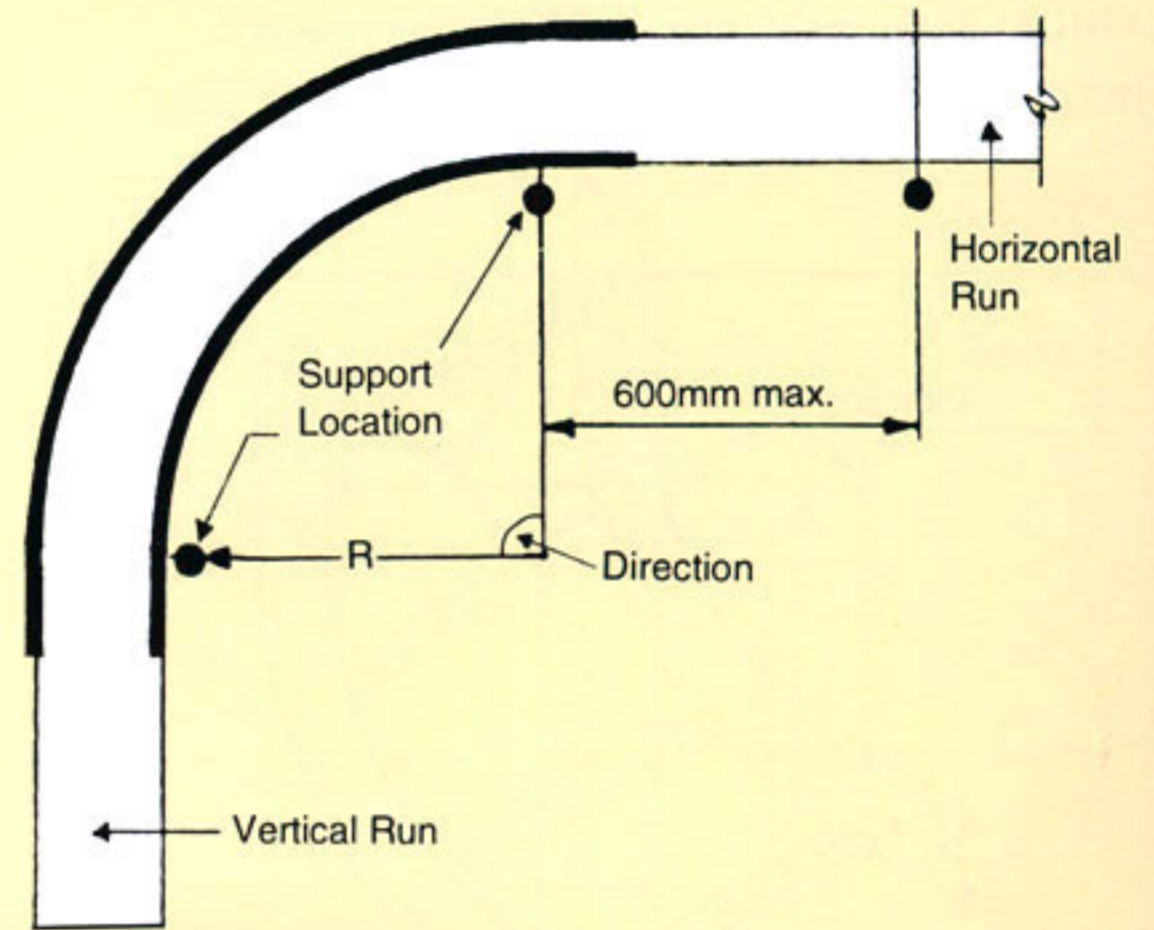
ELEVATIONAL VIEW
