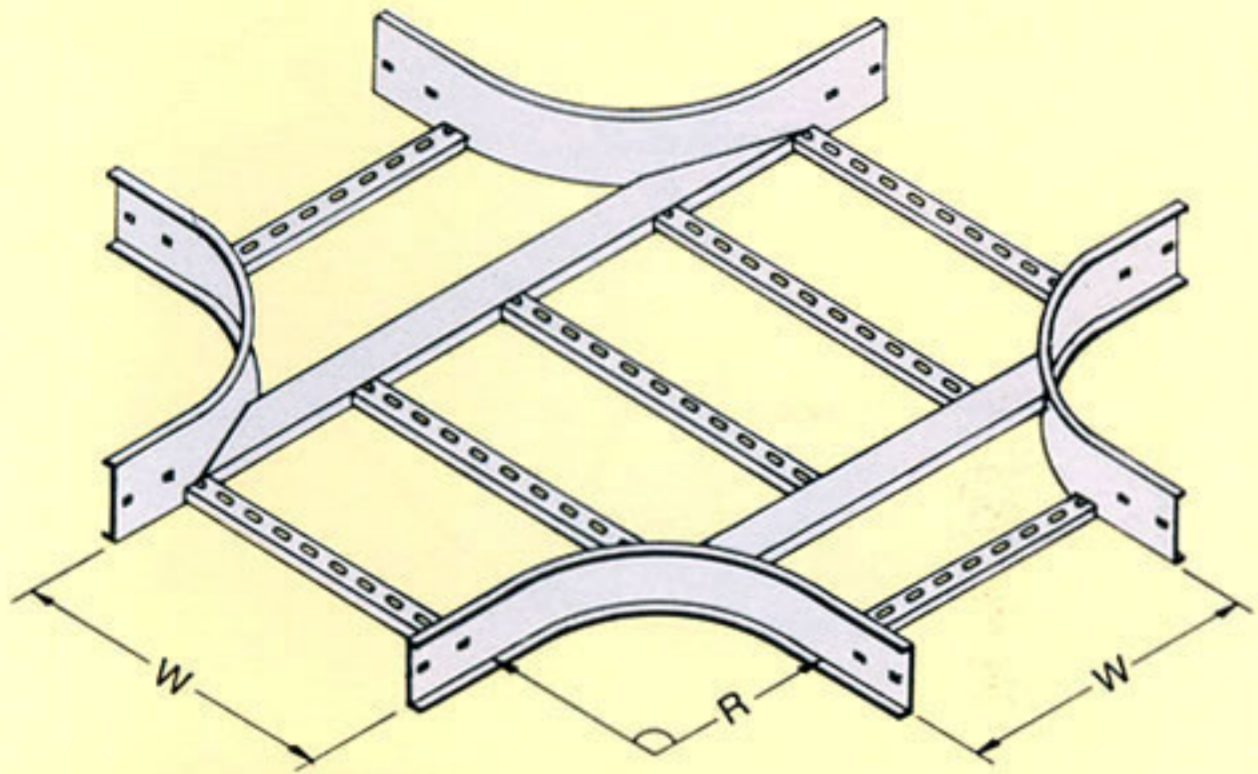
PICTURAL VIEW
