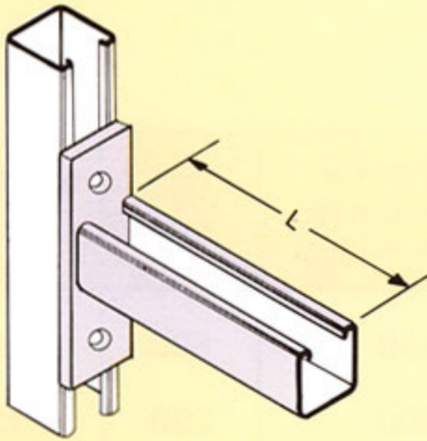
MEDIUM DUTY CANTILEVER BRACKET, ES 2663 SERIES
