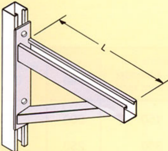
HEAVY DUTY CANTILEVER BRACKET, HCL SERIES
